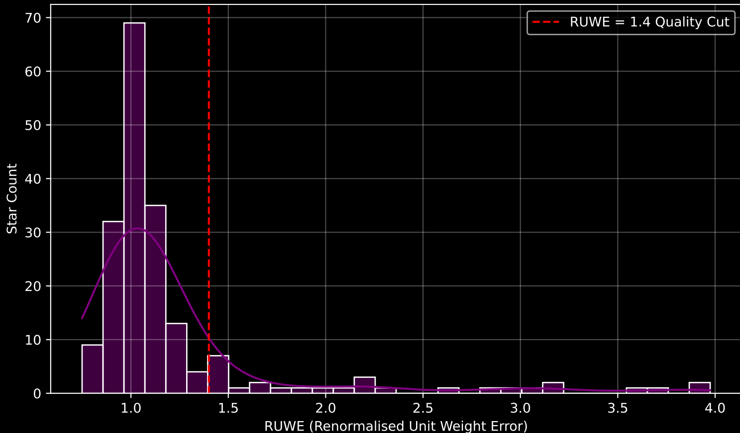
GAPOGEE DR17 Field [186+30] RUWE Distribution (n= 190)
