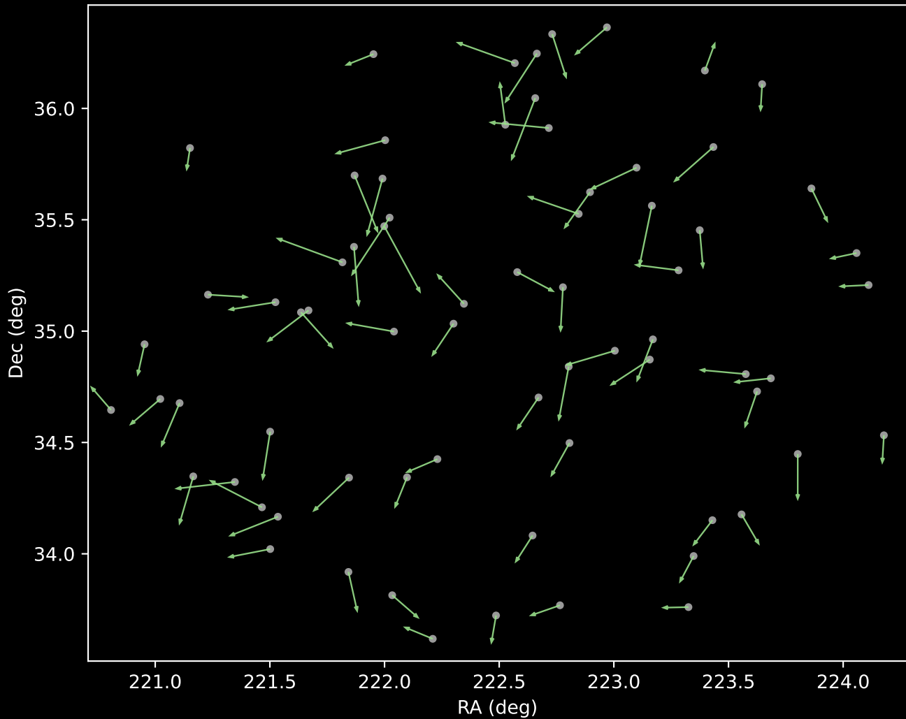
APOGEE DR17 Cluster 5 Proper Motion Vectors (n=71)
