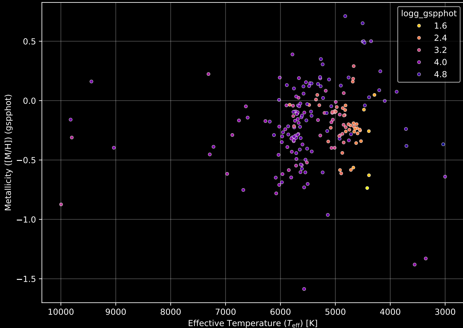
APOGEE DR17 Field: [186+30] Stellar Population Parameters (n= 199)
