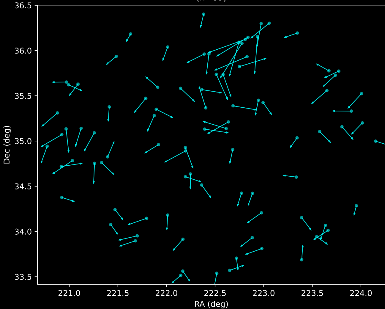
APOGEE DR17 Noise Stream Proper Motion Vectors (n=89)
