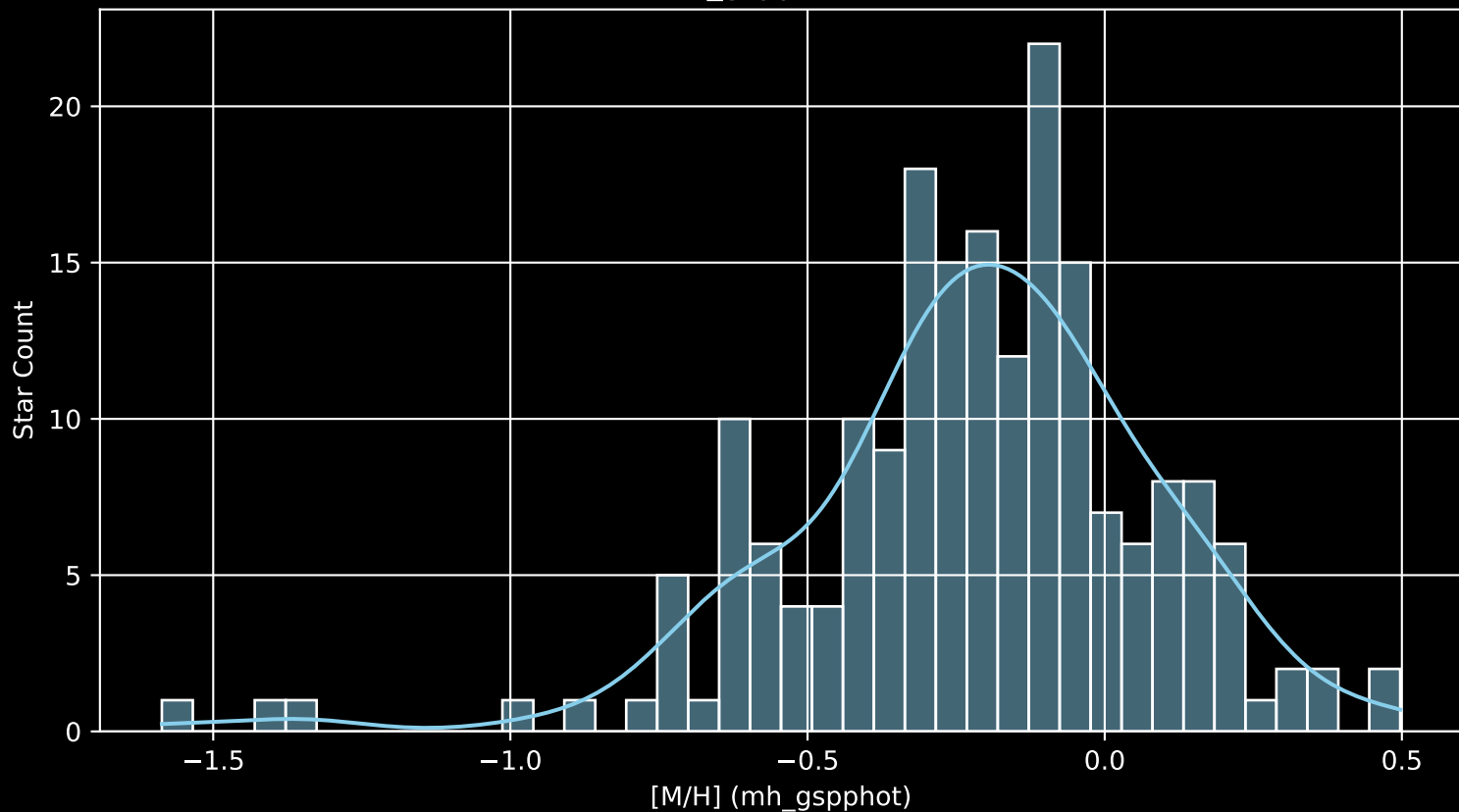
APOGEE DR17 Field: [186+30 [M/H] (mh_gspphot) (n= 195)
