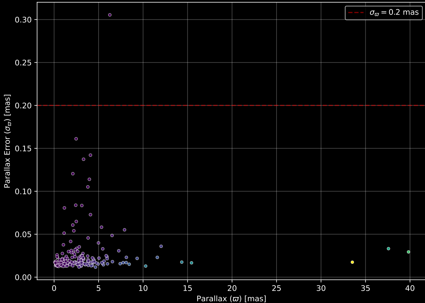
APOGEE DR17 Field: [186+30] Parallax Quality (n= 199)
