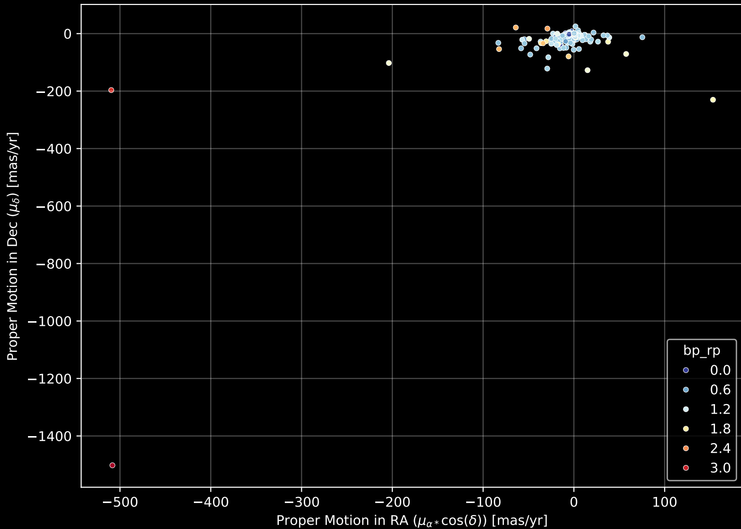
APOGEE DR17 Field: [186+30] Proper Motion Diagram (n= 199)
