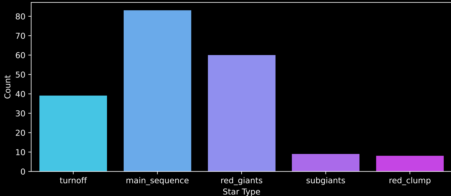
APOGEE DR17 Field: [186+30] Count plot of Star Type
